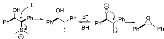
Scheme 3. Possible Invertive Process Yielding trans -3 from cis -1
