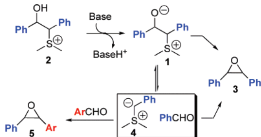
Scheme 2. Probing the Reactivity of Betaine 1 with an Intermolecular Competition Experiment
