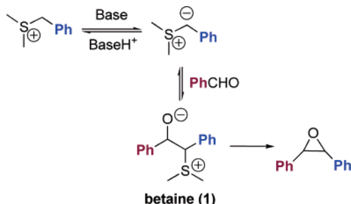
Scheme 1. General Mechanism for the Corey–Chaykovsky Epoxidation Reaction
